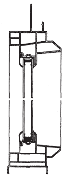
HORIZONTAL MULLER QUARTER ROUNDS WITH THE COUPLER SILL
