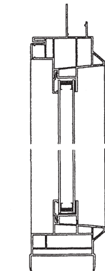
HORIZONTAL MULLED EYEBROWS WITH THE COUPLER SILL
