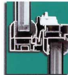
Integral Interlocks
